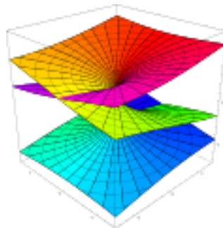
Figure 1: An illustration of a Riemann surface
